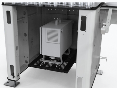
INTEGRATED CONTROLLER COMPARTMENT
